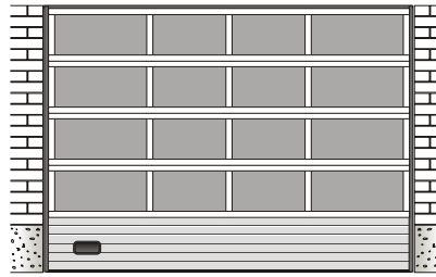
Standard TL-FV door; "Sandwich" type bottom panel
